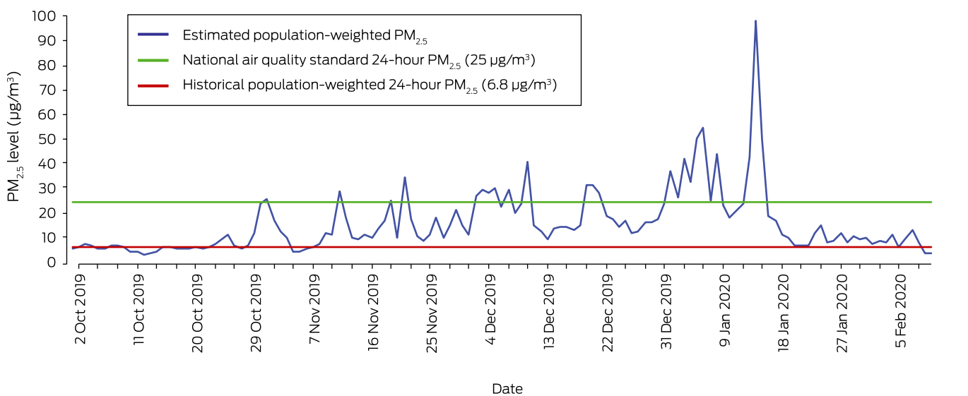
1 Population-weighted \text{PM}_{2.5} levels, New South Wales, Queensland, the Australian Capital Territory and Victoria, 1 October 2019 – 10 February 2020*
